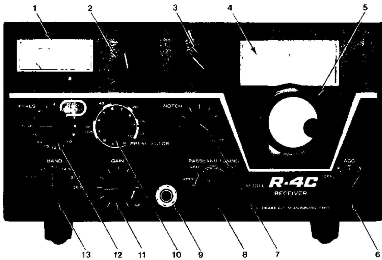
Figure 3-1 Front Panel Controls
