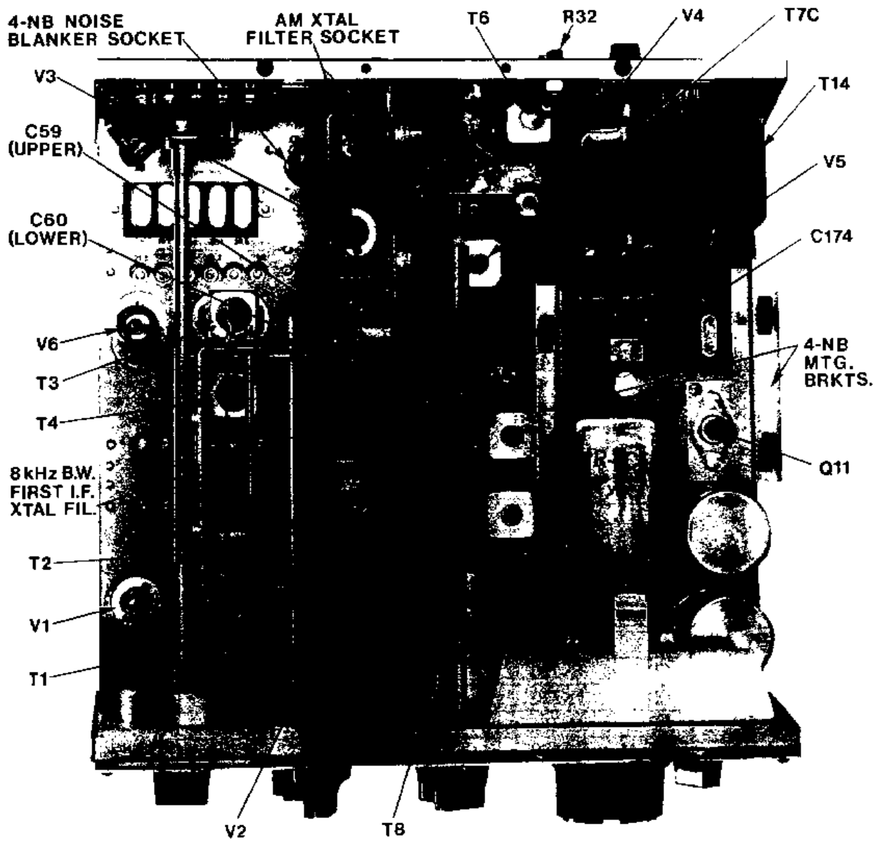
Figure 5-1. Alignment Locations, Top View
