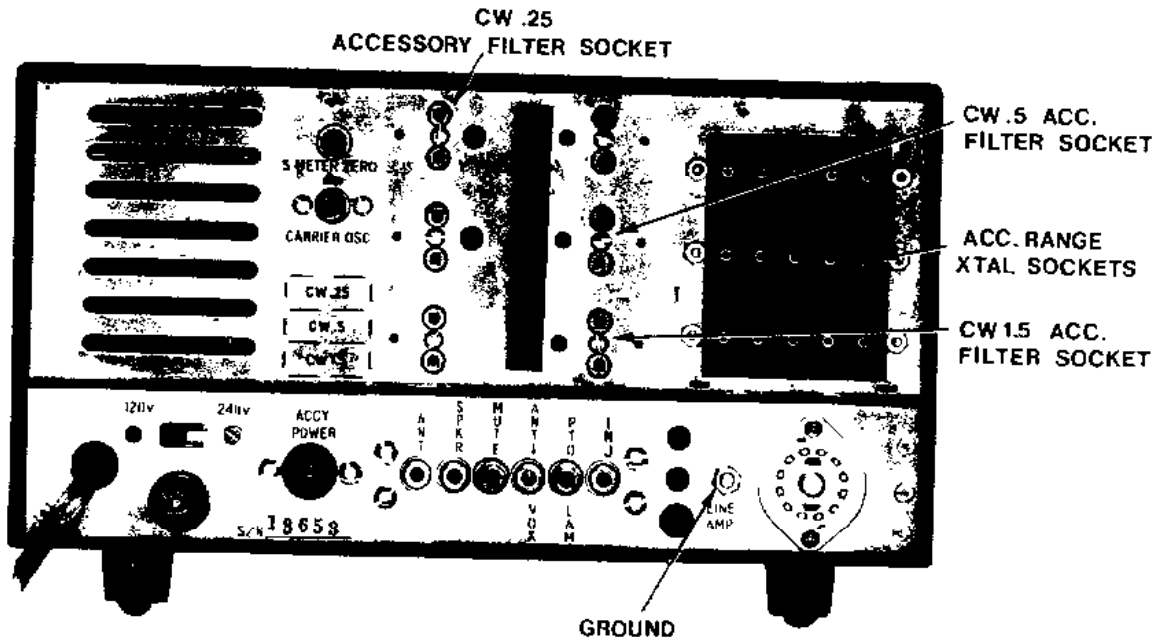
Figure 2-2. Rear Chassis Controls
