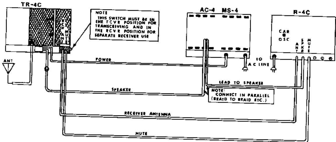
Figure 2-3 Connecting the TR-4C Transceiver
