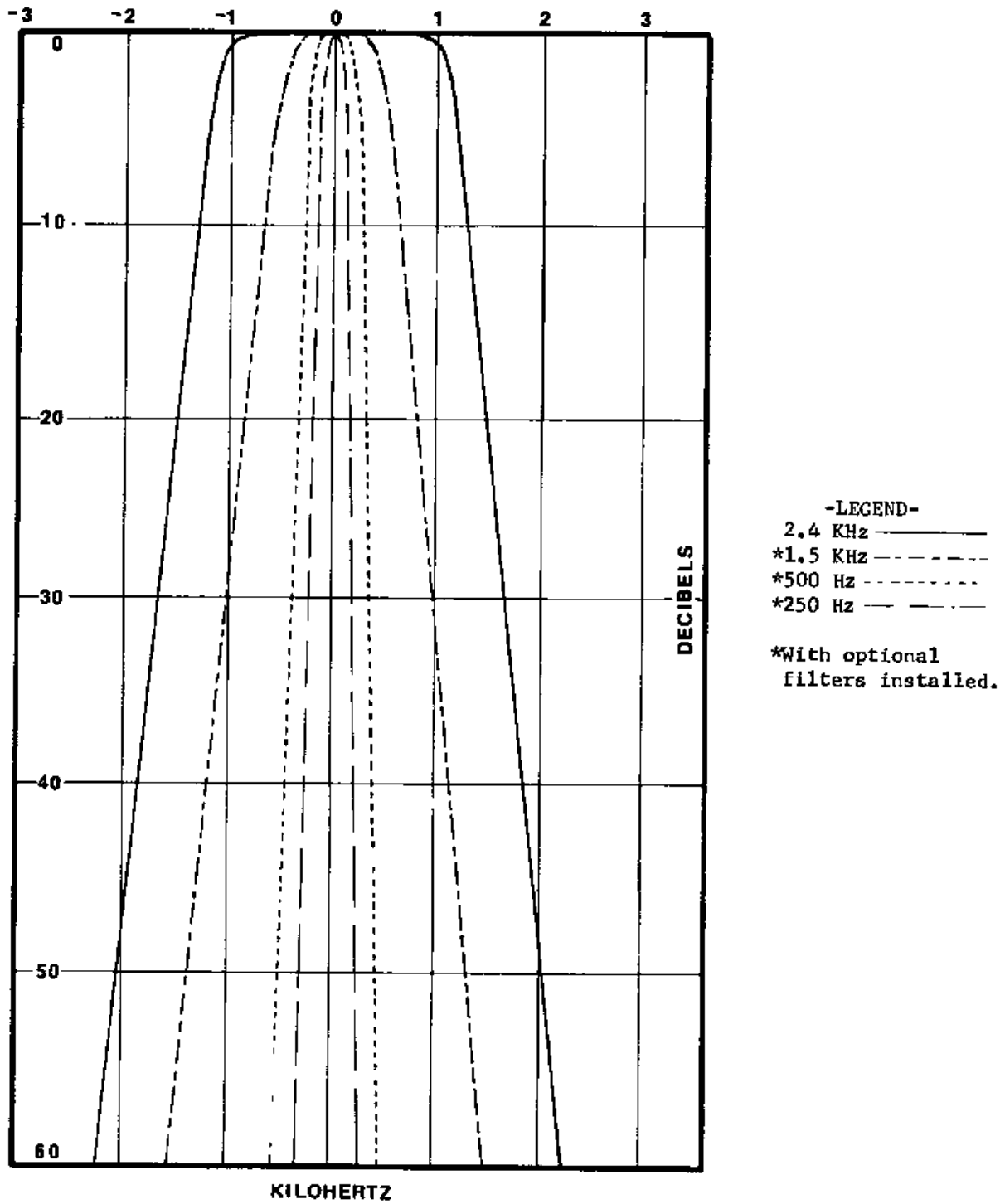
Figure 3-4. SSB and CW Selectivity Curves
