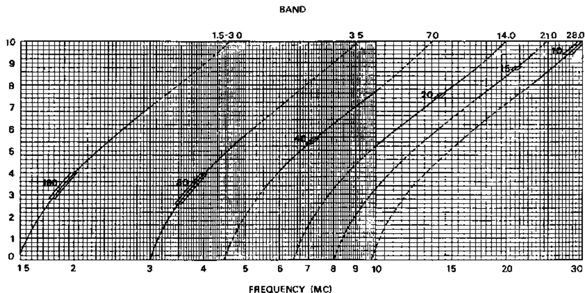
Figure 3-2 Preselector Tuning Ranges
