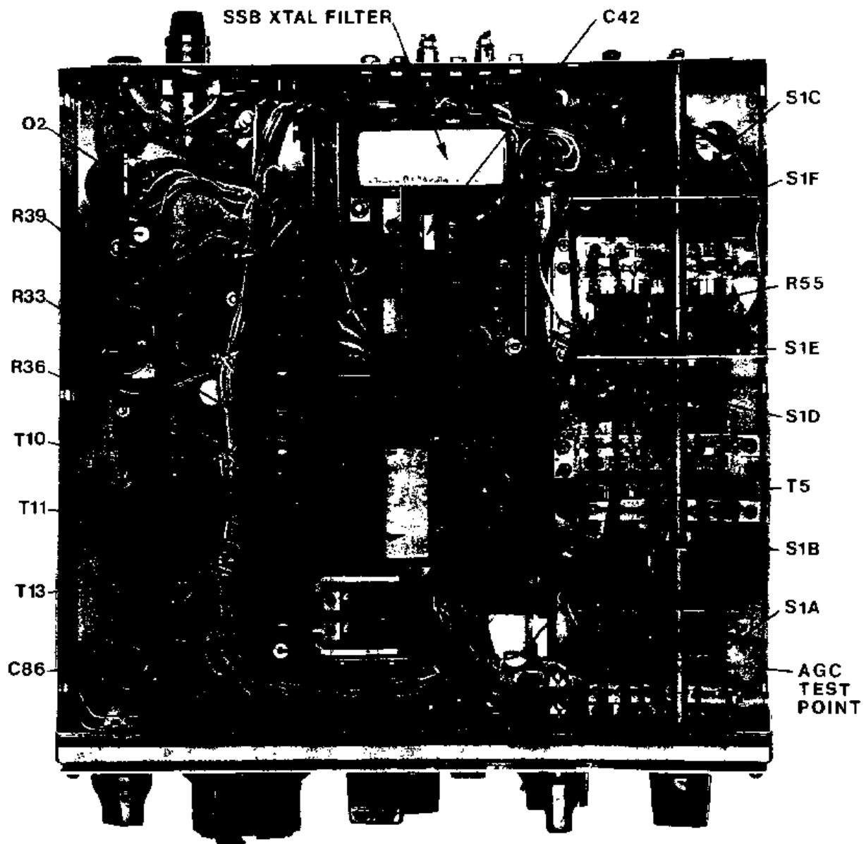
Figure 5-2. Alignment Locations, Bottom View
