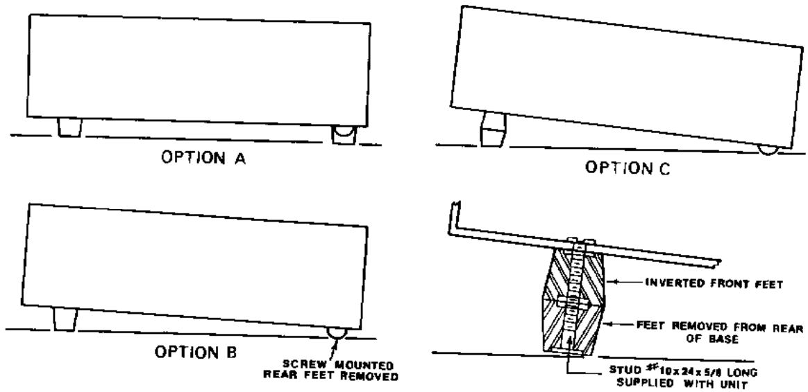
Figure 2-1. Viewing Angle Options
