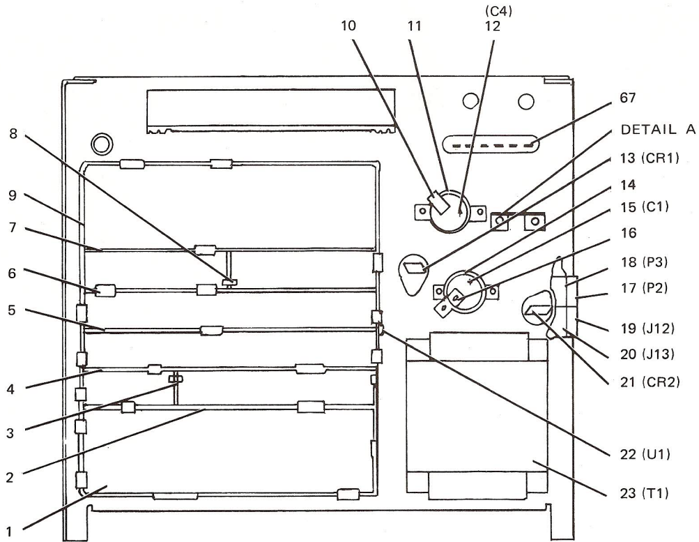
TOP VIEW
